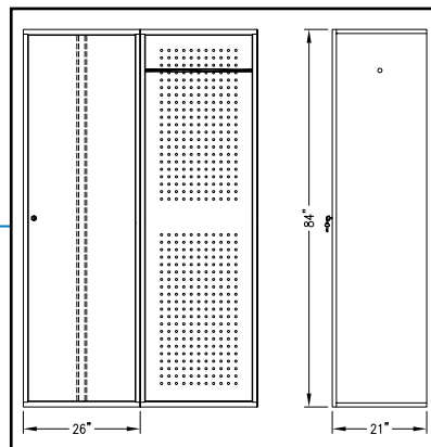
Bulky Garment Disposal: 26" x 21" x 84"
