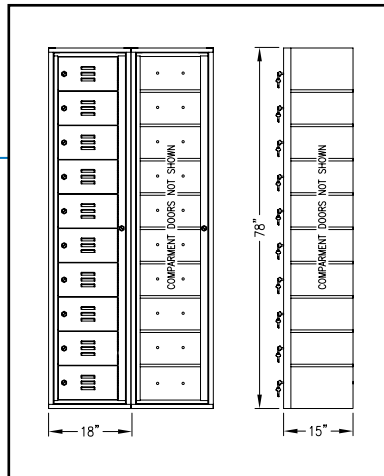
10-Compartment Folded: 18" x 15" x 78"
