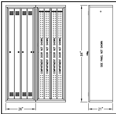
4-Compartment Long Hanging: 26" x 21" x 84"
