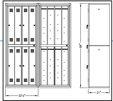
8-Compartment Wide Hanging: 32½" x 21" x 84"
