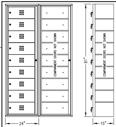
9-Compartment Folded: 24" x 15" x 81"
