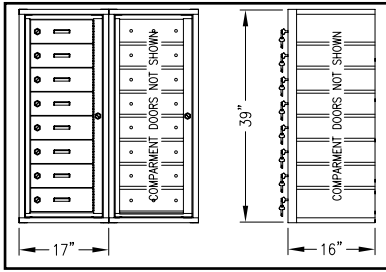
8-Compartment Mini Folded: 17" x 16" x 39"
