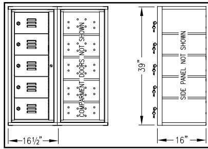
5-Compartment Folded: 17" x 16" x 39"
