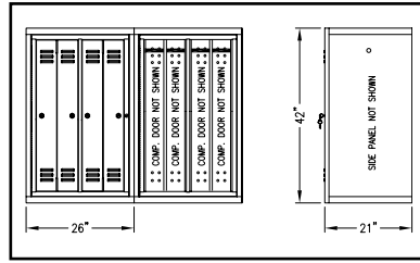
4-Compartment Mini Hanging: 26" x 21" x 42"
