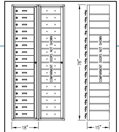
16-Compartment Folded: 18" x 15" x 78"
