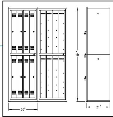
8-Compartment Hanging: 26" x 21" x 84"
