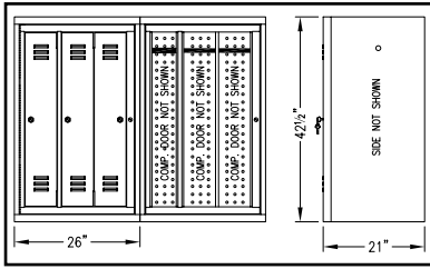
3-Compartment Hanging: 26" x 21" x 42½"
