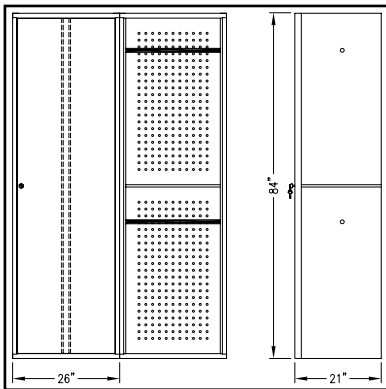
Linen Exchange: 26" x 21" x 84"
