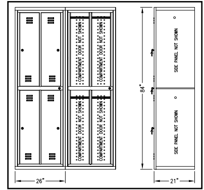
4-Compartment Hanging: 26" x 21" x 84"
